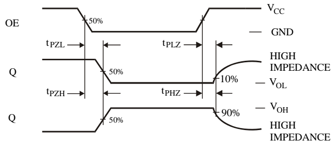
Figure 2. Switching Waveforms
